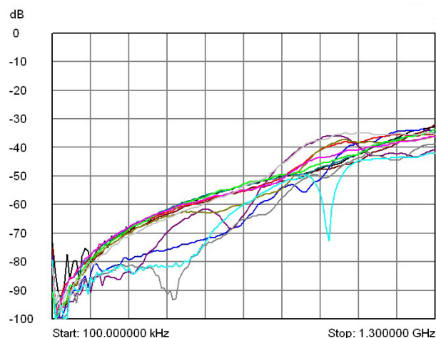
40-749-511/521 (50 \Omega ) Typical crosstalk between channels (these are measurements of crosstalk within each multiplexer for neighboring channels).
