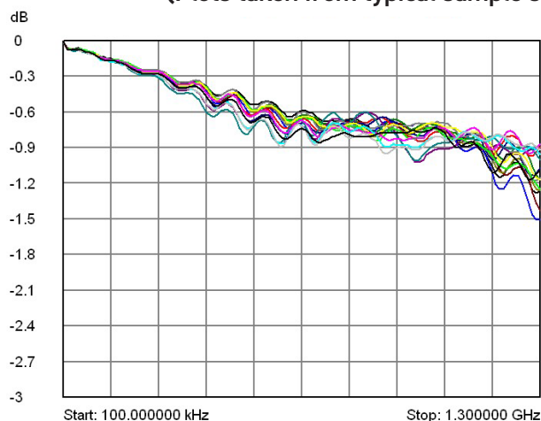
40-749-511/521 (50 \Omega ) Typical insertion loss plots for each channel.
