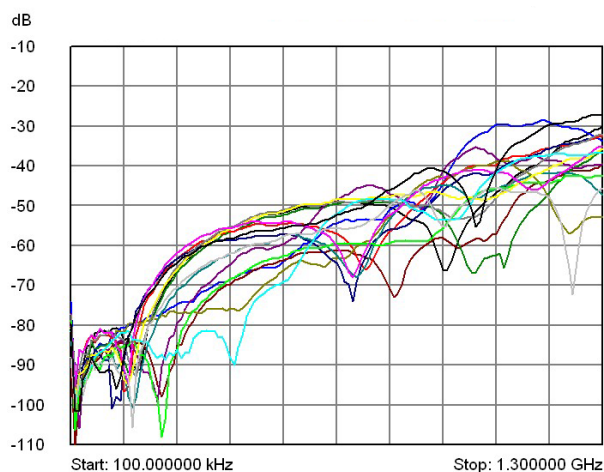
40-749-511/521 (50 \Omega ) Typical Isolation Plots for each input channel.
