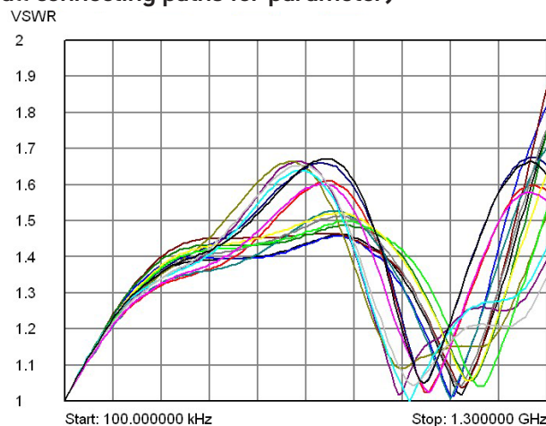
40-749-511/521 (50 \Omega ) Typical VSWR plots for each channel.
