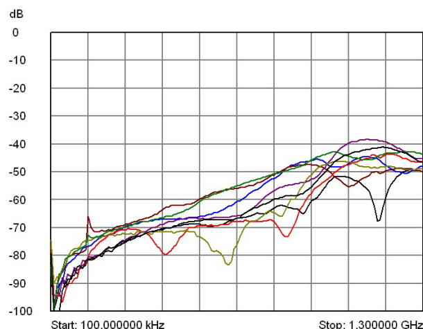
40-749-511/521 (50 \Omega ) Typical crosstalk between MUX banks (these are measurements of crosstalk between the same paths through neighboring multiplexers).
